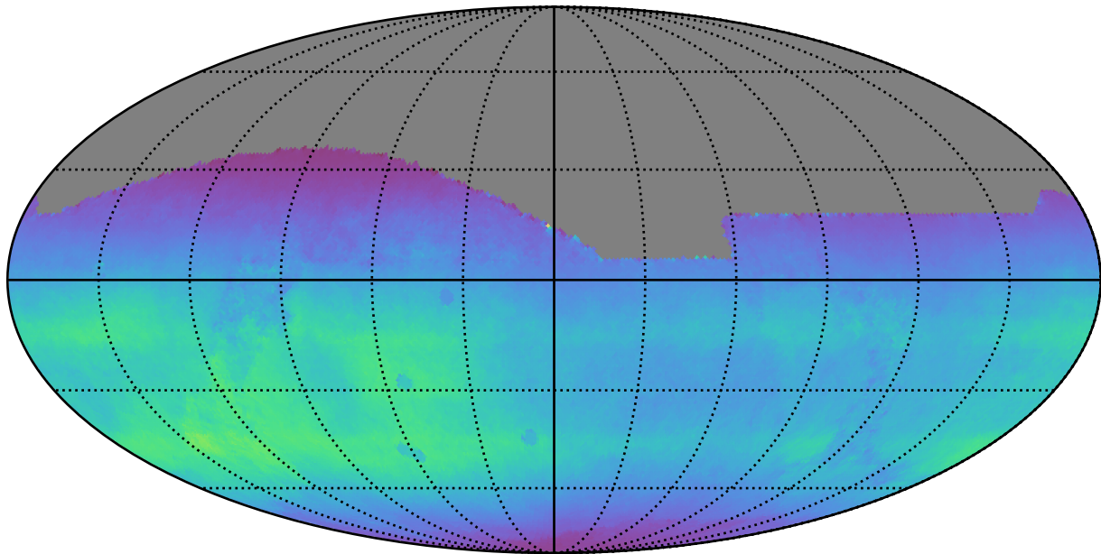
too_ignore_5_4v3.4_10yrs All sky all bands: Normalized Teff
