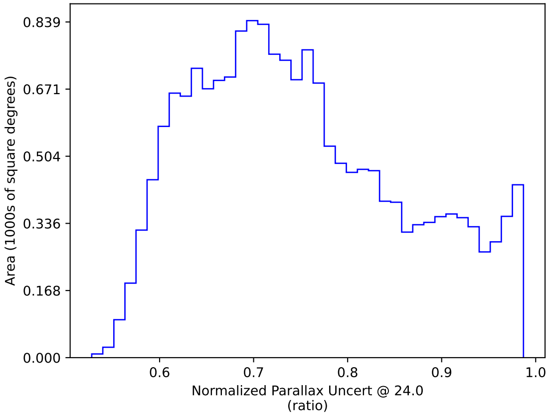
too_ignore_5_4v3.4_10yrs WFD: Normalized Parallax Uncert @ 24.0
