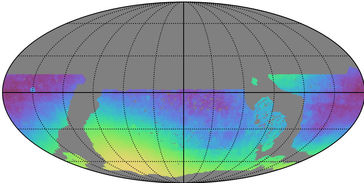
too_ignore_5_4v3.4_10yrs WFD: Normalized Parallax Uncert @ 22.4
