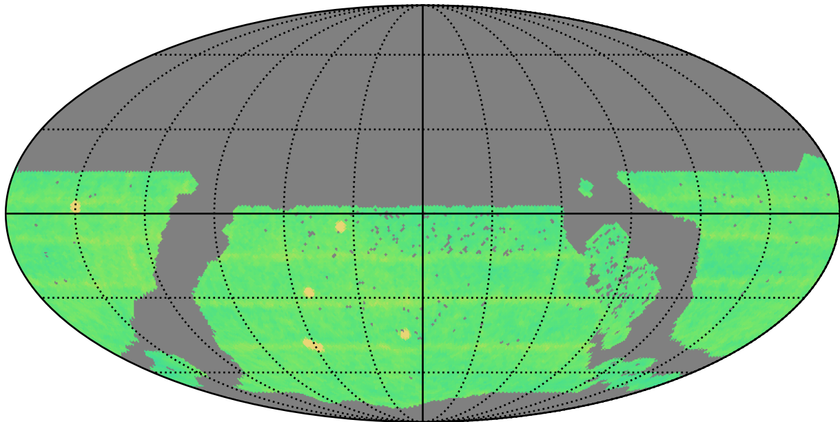
too_ignore_5_4v3.4_10yrs WFD all bands: N Unique Nights
