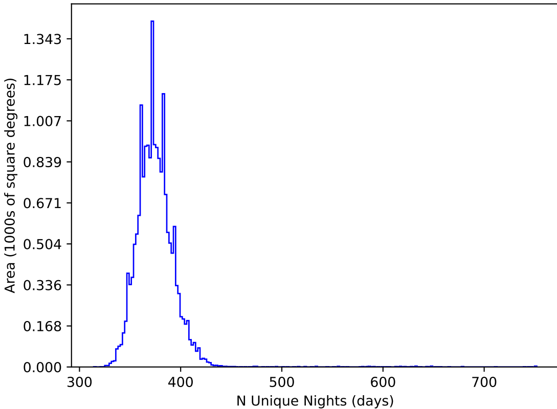
too_ignore_5_4v3.4_10yrs WFD all bands: N Unique Nights
