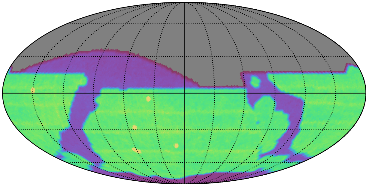
too_ignore_5_4v3.4_10yrs All sky all bands: N Unique Nights
