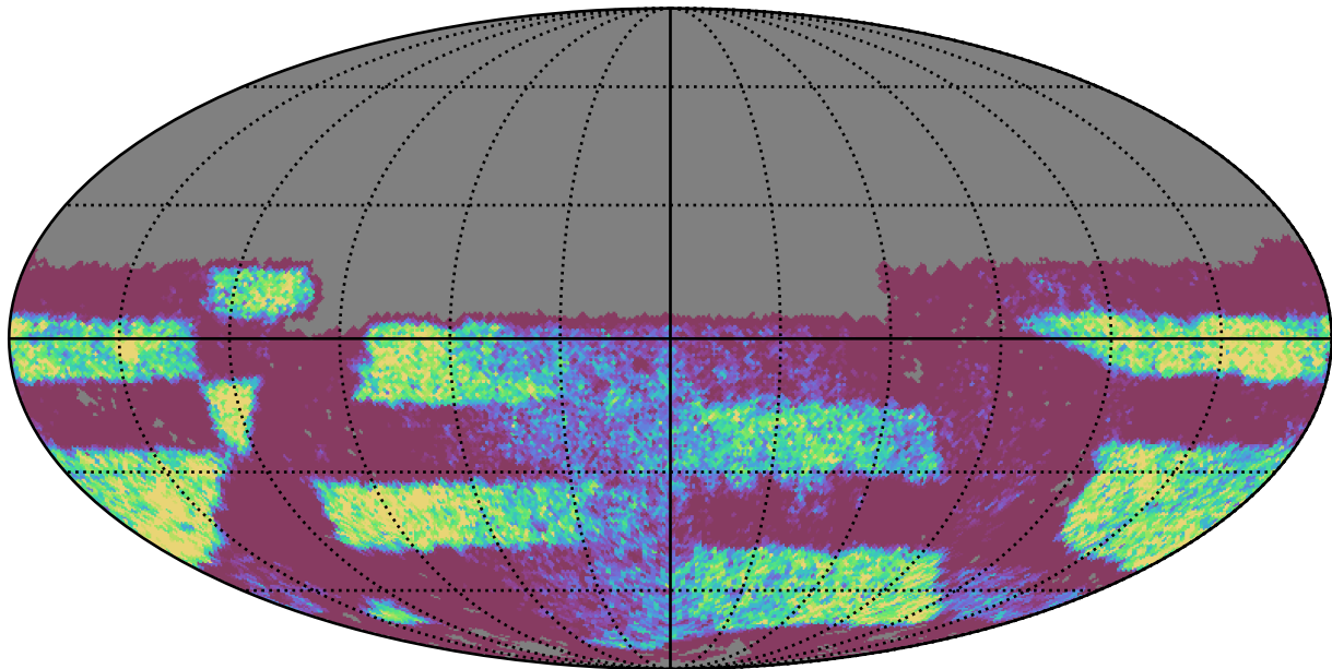
too_ignore_5_4v3.4_10yrs Yr 3-4 y band: NVisits
