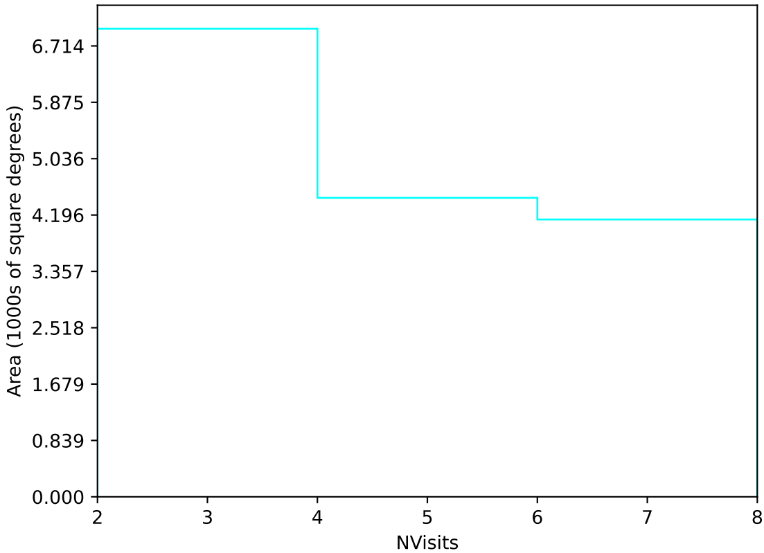
too_ignore_5_4v3.4_10yrs Yr 3-4 u band: NVisits
