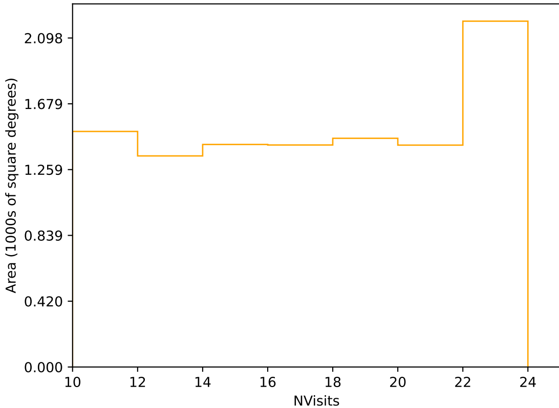
too_ignore_5_4v3.4_10yrs Yr 3-4 r band: NVisits
