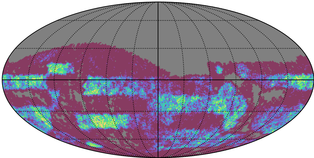
too_ignore_5_4v3.4_10yrs Yr 3-4 g band: NVisits
