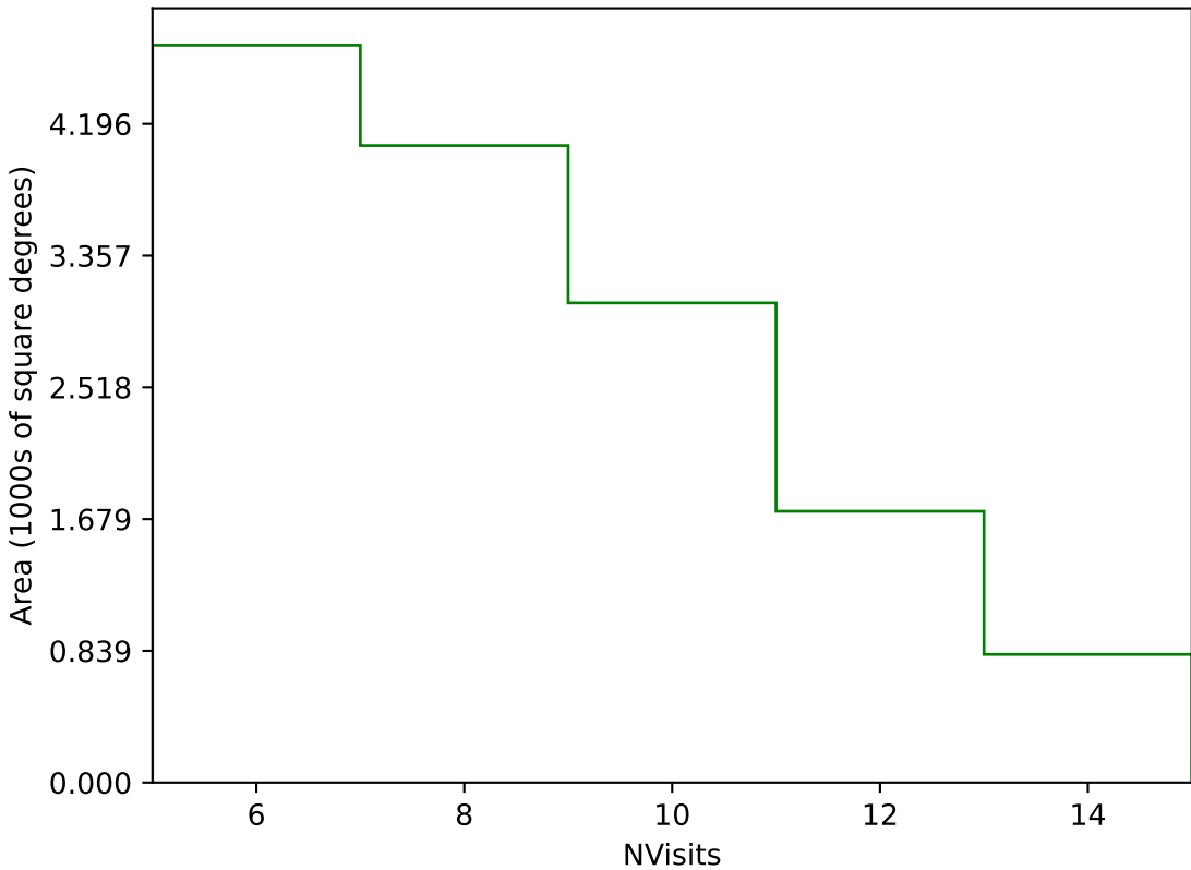
too_ignore_5_4v3.4_10yrs Yr 3-4 g band: NVisits
