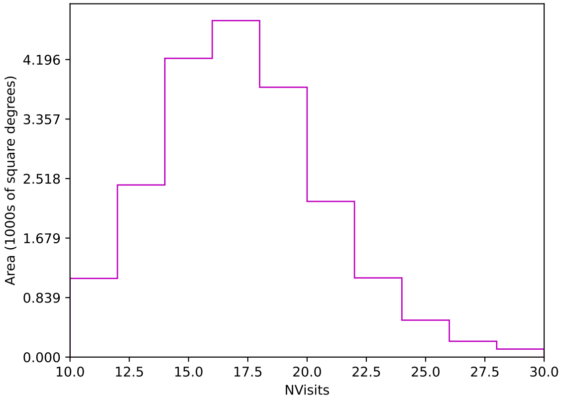
too_ignore_5_4v3.4_10yrs Yr 1 z band: NVisits
