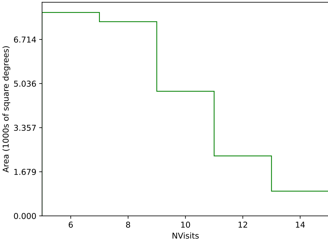
too_ignore_5_4v3.4_10yrs Yr 1 g band: NVisits
