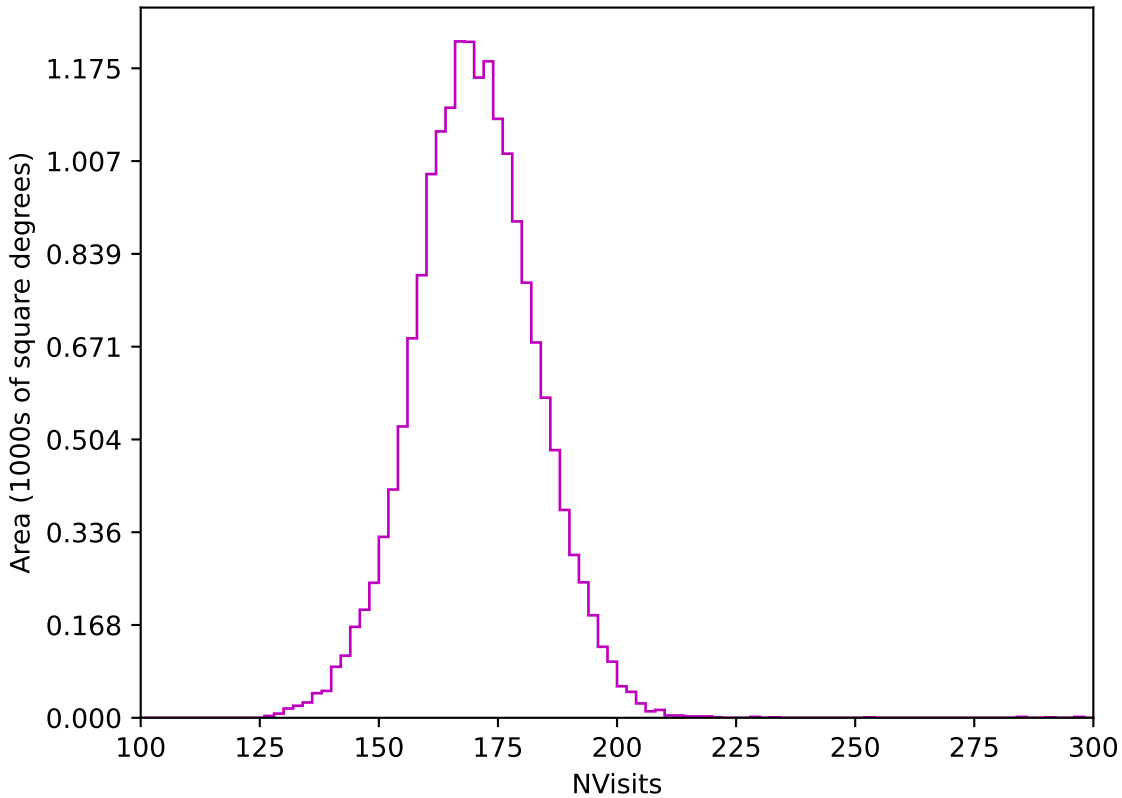
too_ignore_5_4v3.4_10yrs WFD z band: NVisits
