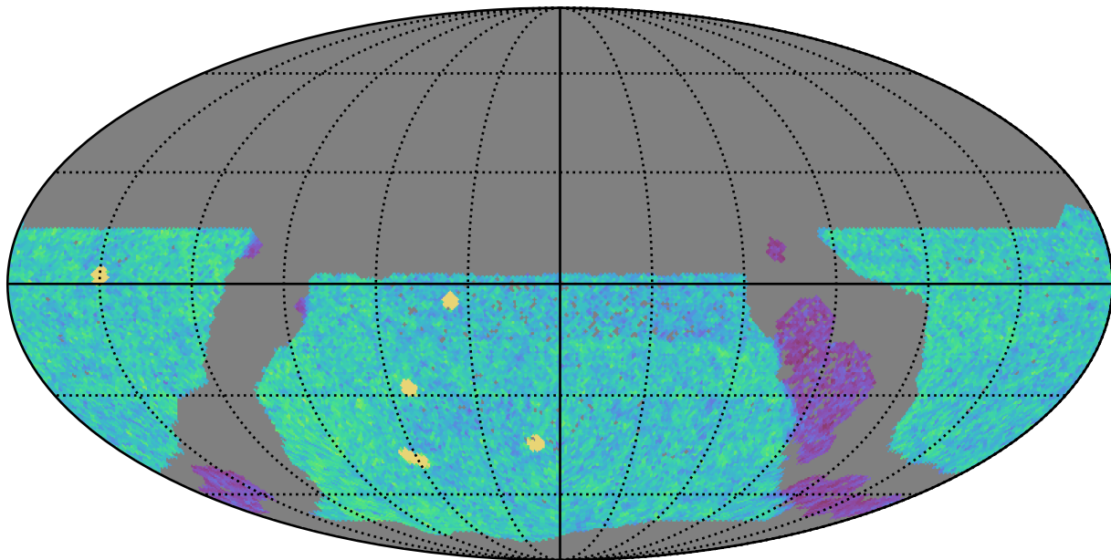
too_ignore_5_4v3.4_10yrs WFD u band: NVisits
