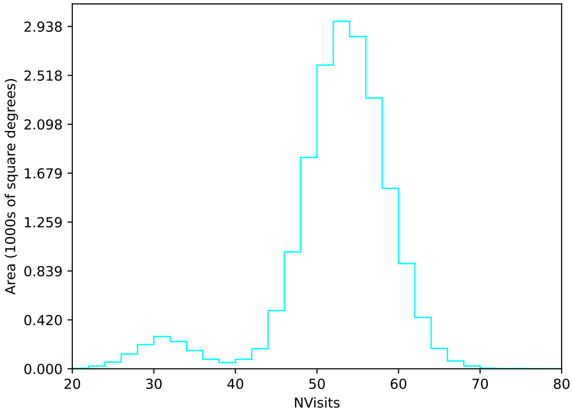
too_ignore_5_4v3.4_10yrs WFD u band: NVisits
