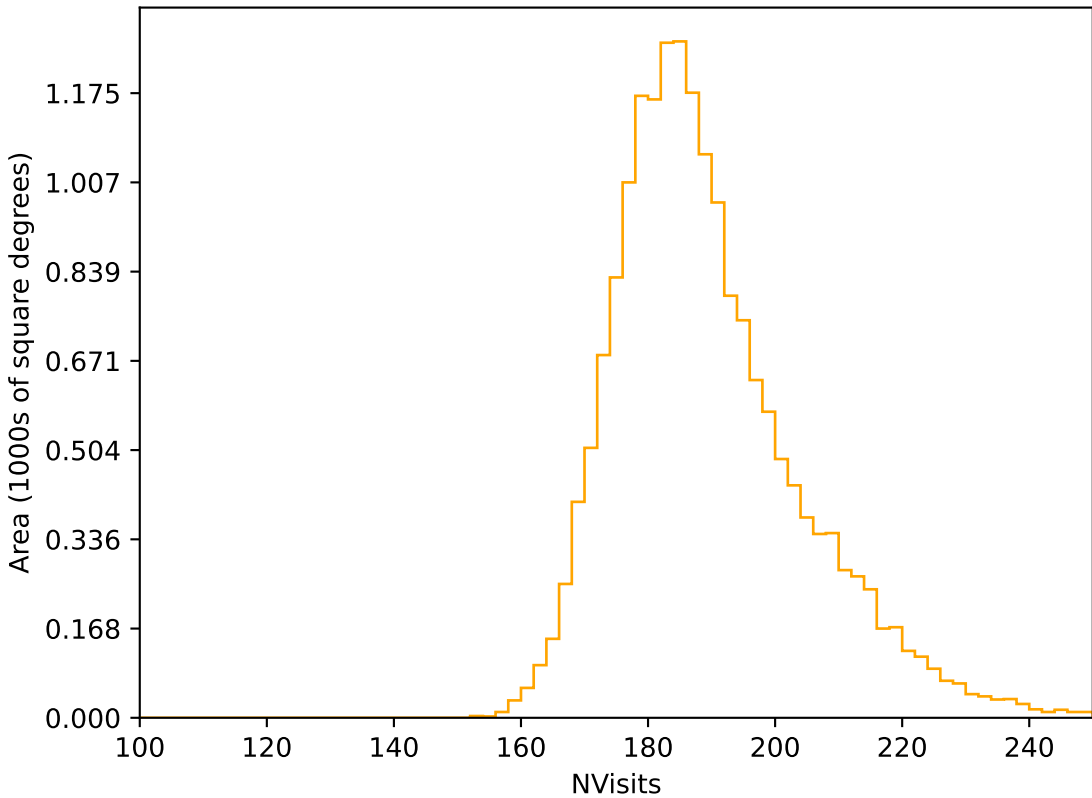
too_ignore_5_4v3.4_10yrs WFD r band: NVisits
