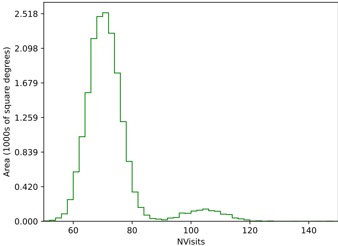
too_ignore_5_4v3.4_10yrs WFD g band: NVisits
