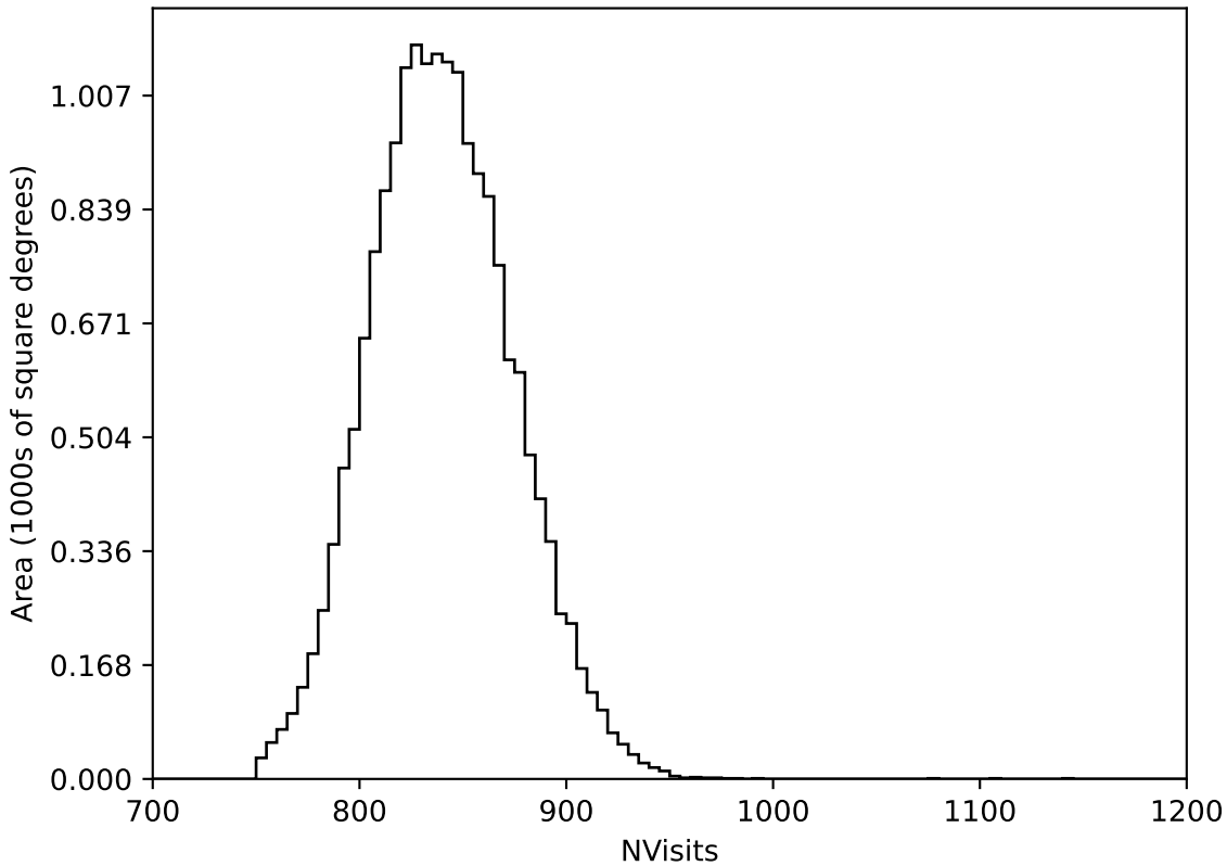
too_ignore_5_4v3.4_10yrs WFD all bands: NVisits
