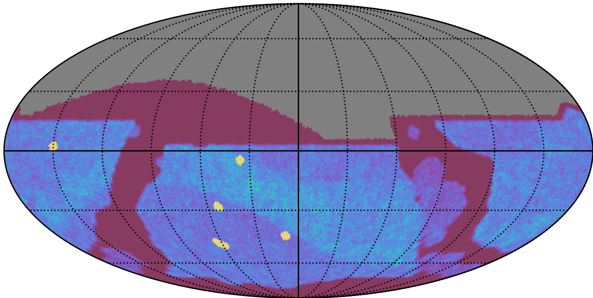
too_ignore_5_4v3.4_10yrs All sky z band: NVisits
