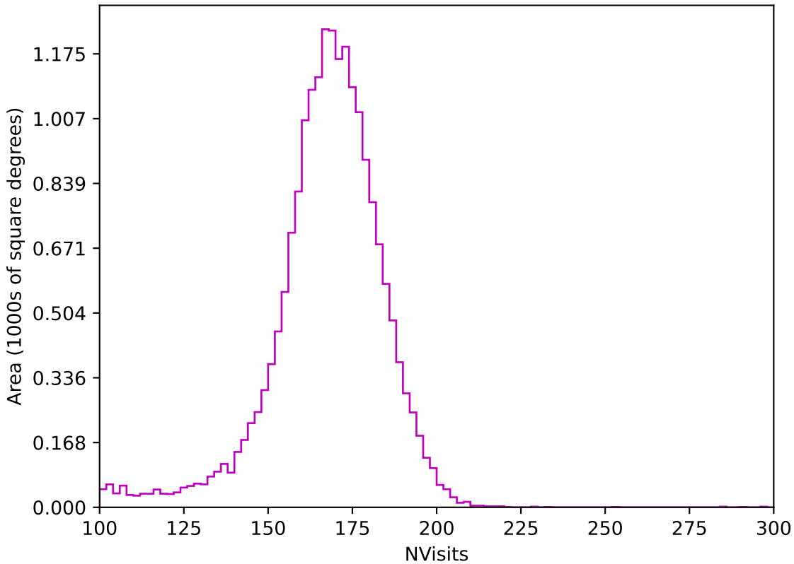
too_ignore_5_4v3.4_10yrs All sky z band: NVisits
