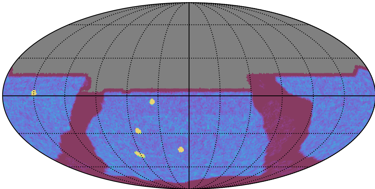
too_ignore_5_4v3.4_10yrs All sky y band: NVisits
