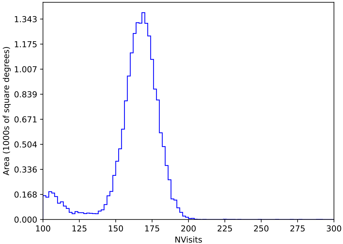
too_ignore_5_4v3.4_10yrs All sky y band: NVisits
