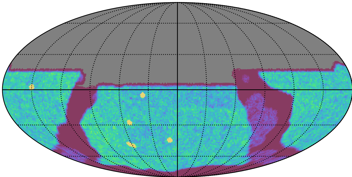
too_ignore_5_4v3.4_10yrs All sky u band: NVisits
