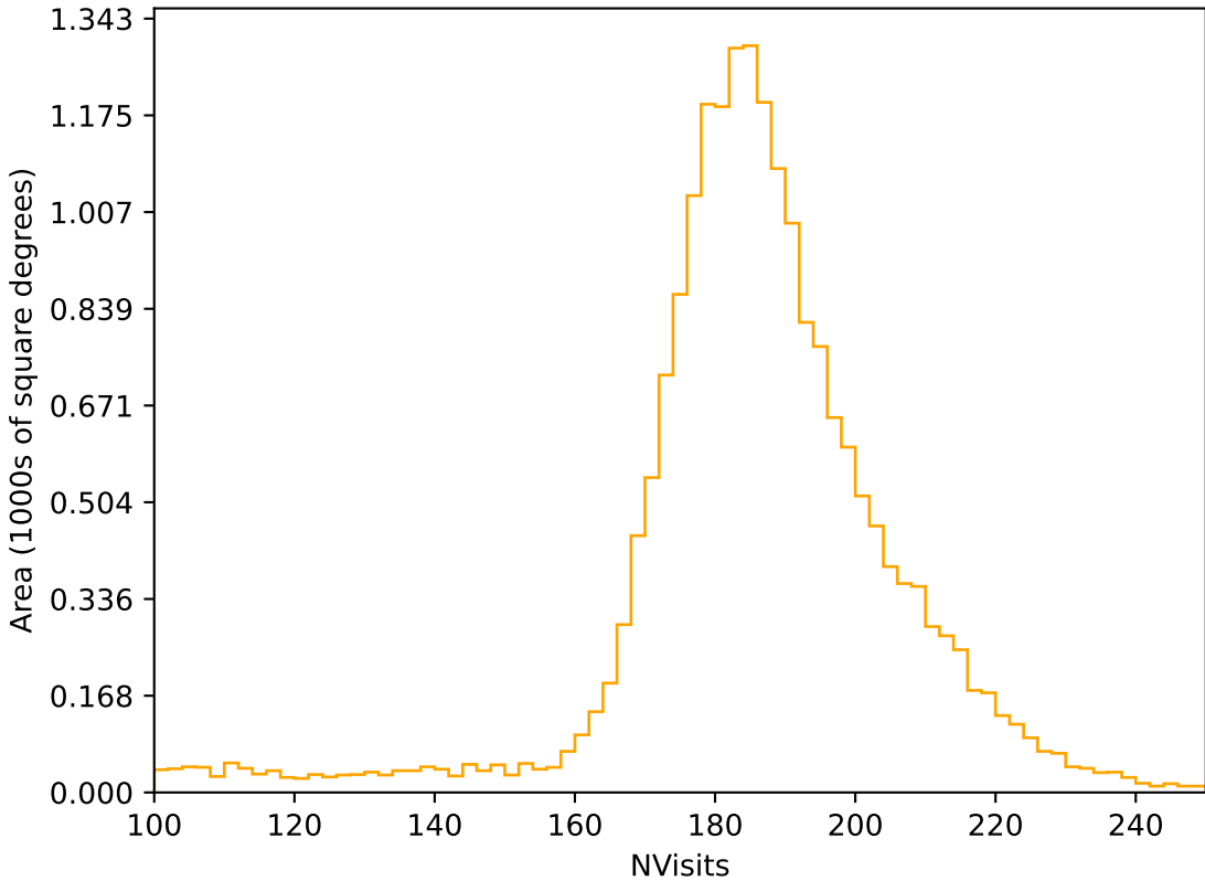
too_ignore_5_4v3.4_10yrs All sky r band: NVisits
