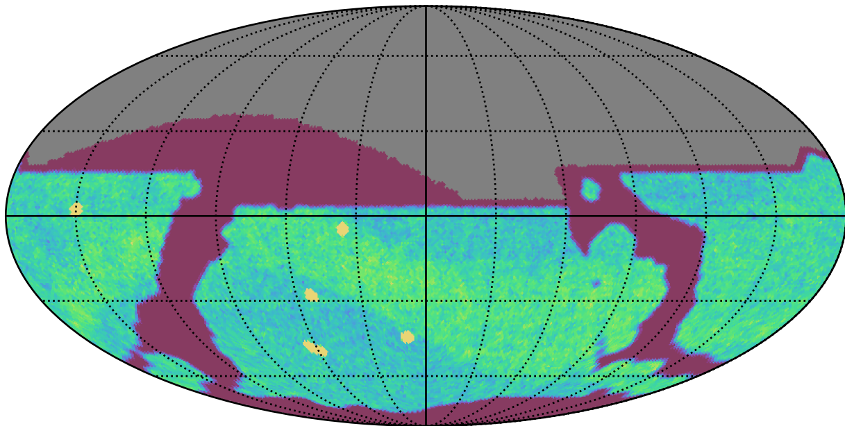
too_ignore_5_4v3.4_10yrs All sky i band: NVisits
