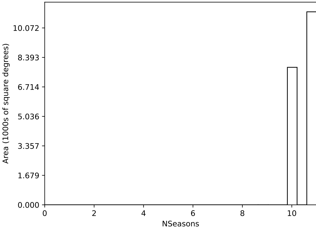
too_ignore_5_4v3.4_10yrs WFD all bands: NSeasons
