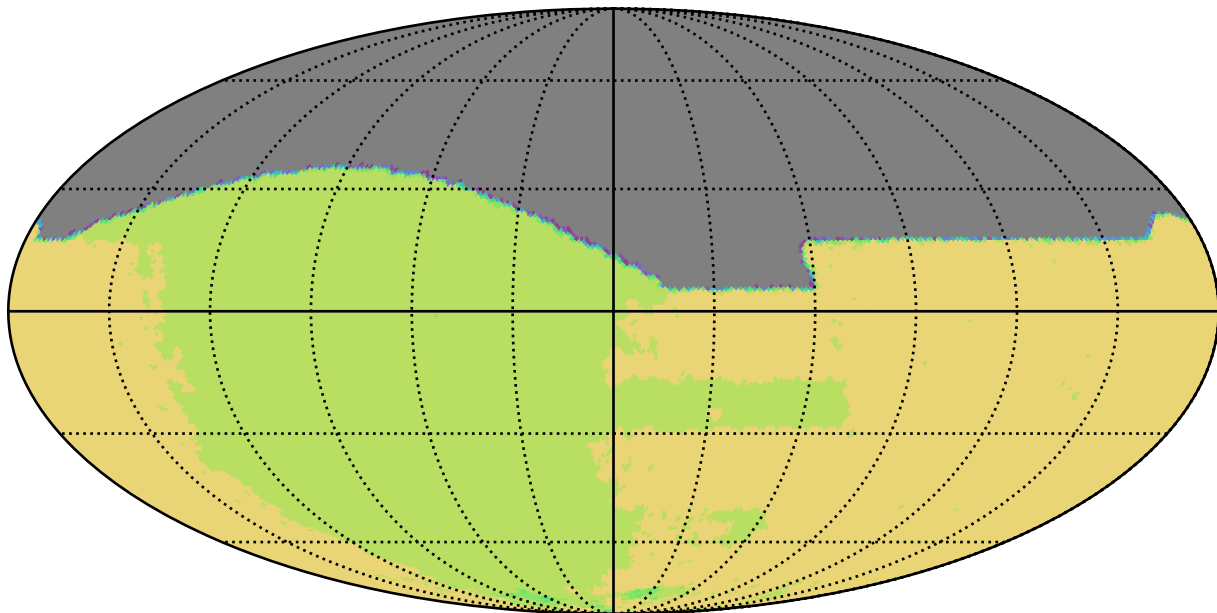
too_ignore_5_4v3.4_10yrs All sky all bands: NSeasons
