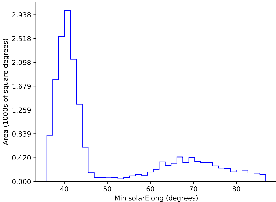
too_ignore_5_4v3.4_10yrs WFD i band: Min solarElong
