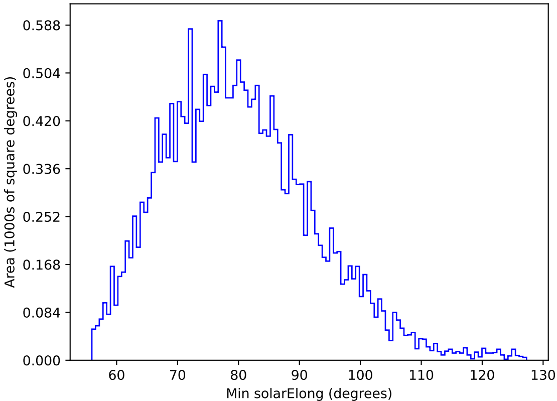
too_ignore_5_4v3.4_10yrs All sky u band: Min solarElong
