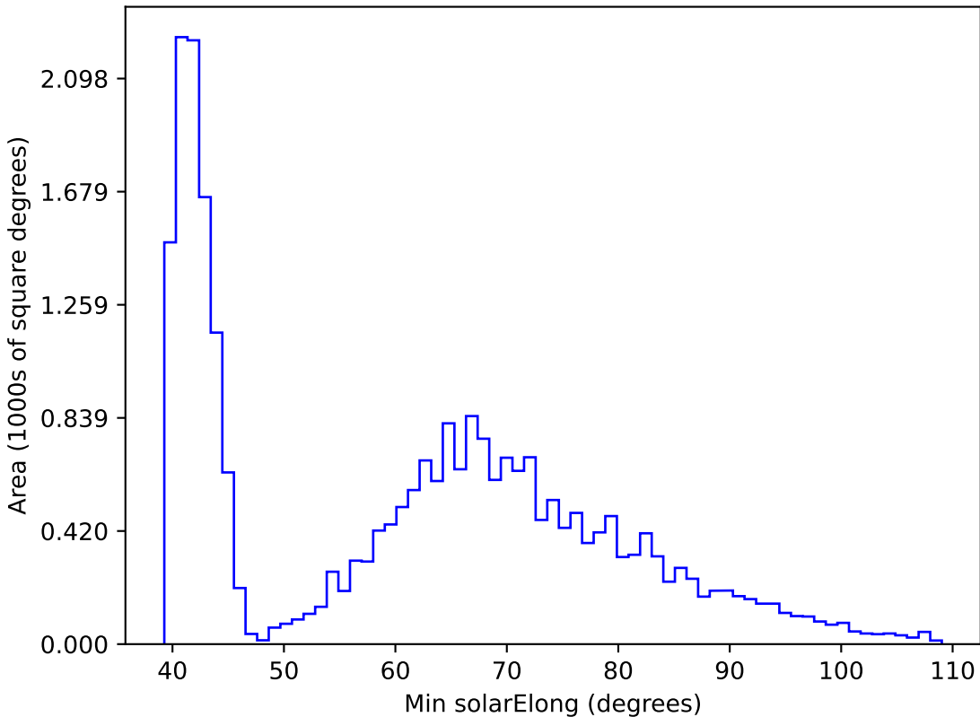
too_ignore_5_4v3.4_10yrs All sky r band: Min solarElong
