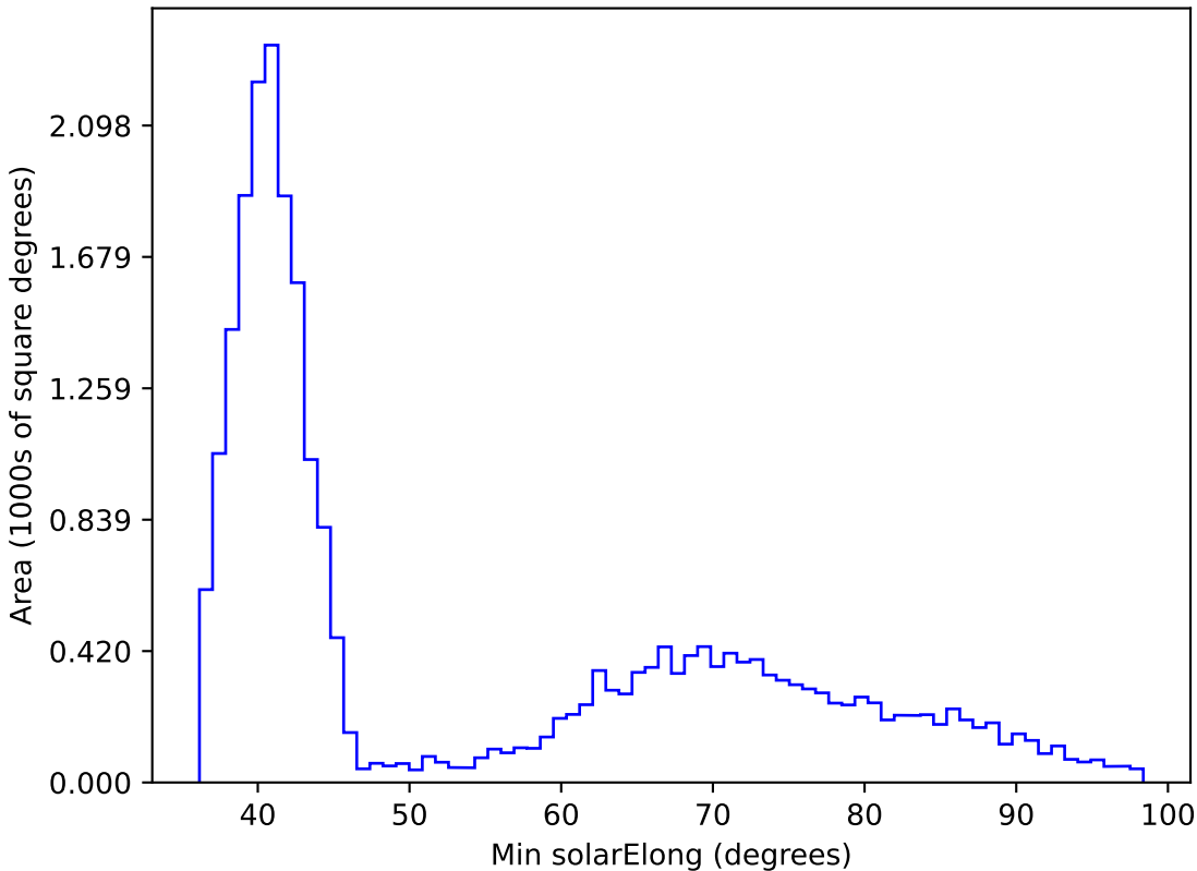
too_ignore_5_4v3.4_10yrs All sky i band: Min solarElong
