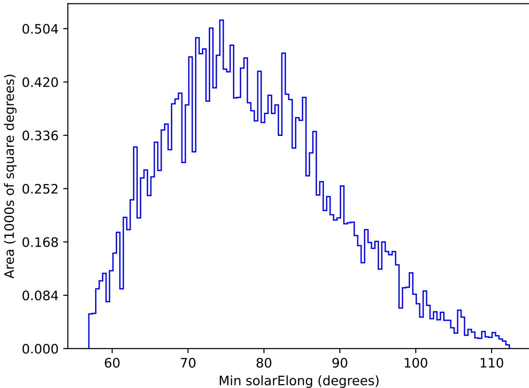
too_ignore_5_4v3.4_10yrs All sky g band: Min solarElong
