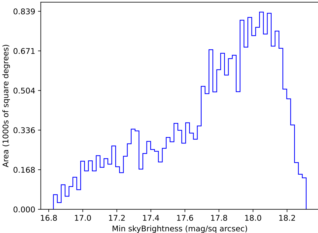
too_ignore_5_4v3.4_10yrs Yr 1 y band: Min skyBrightness
