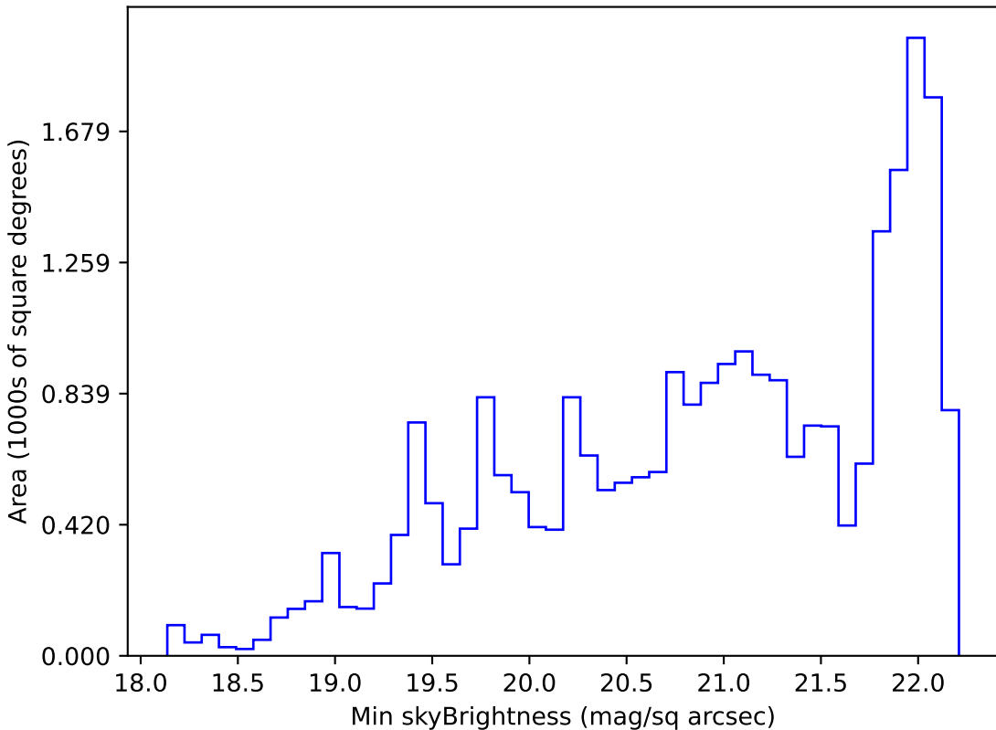
too_ignore_5_4v3.4_10yrs Yr 1 g band: Min skyBrightness
