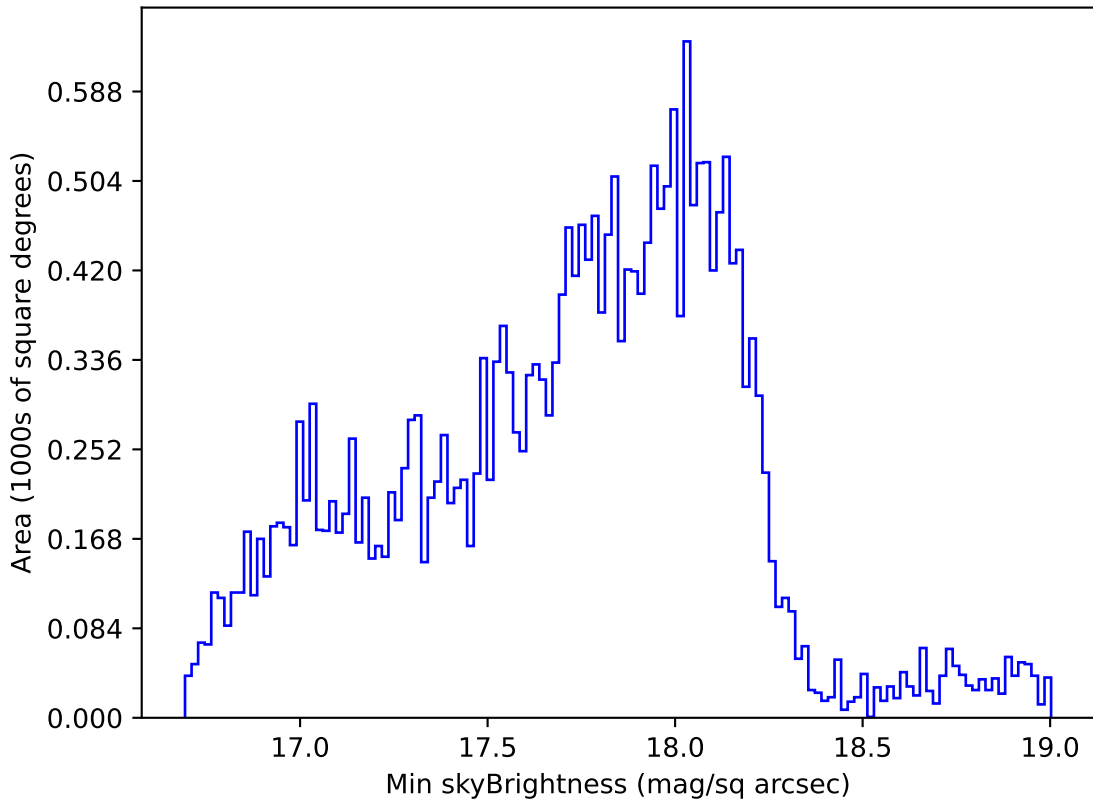
too_ignore_5_4v3.4_10yrs Yr 1 all bands: Min skyBrightness
