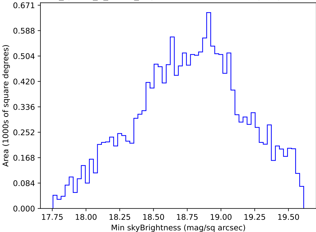
too_ignore_5_4v3.4_10yrs WFD r band: Min skyBrightness
