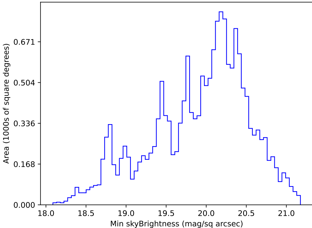
too_ignore_5_4v3.4_10yrs WFD g band: Min skyBrightness
