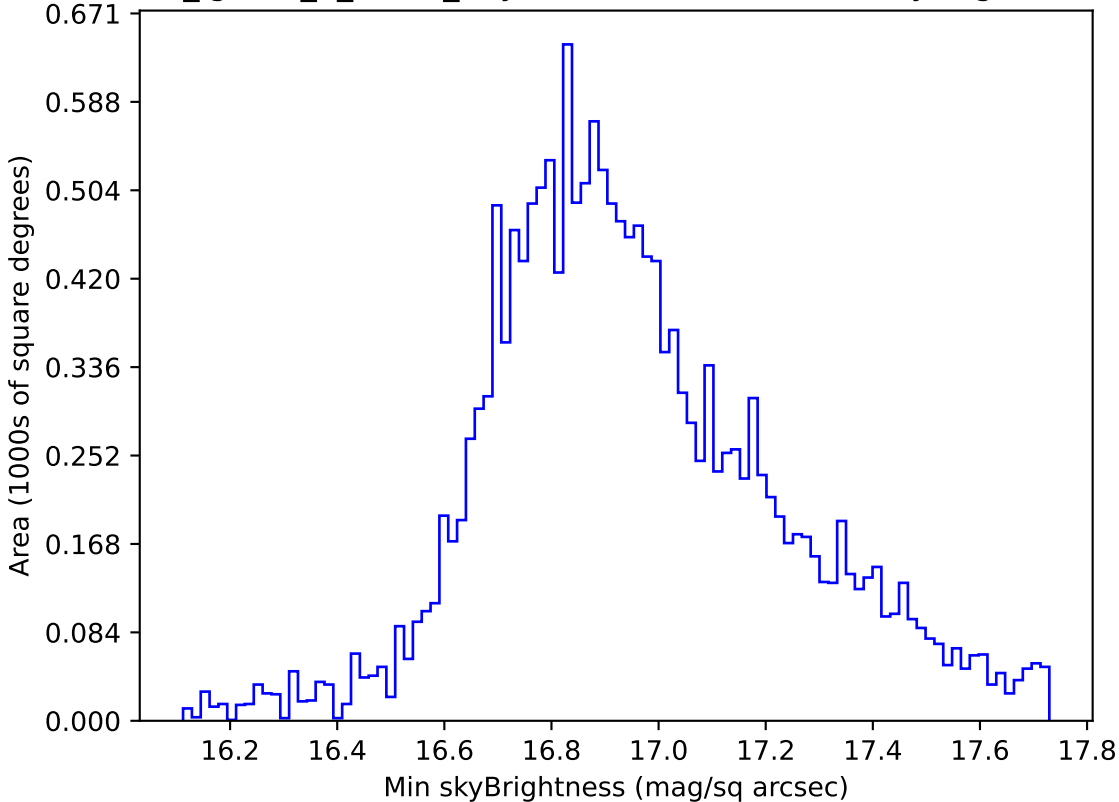
too_ignore_5_4v3.4_10yrs WFD all bands: Min skyBrightness
