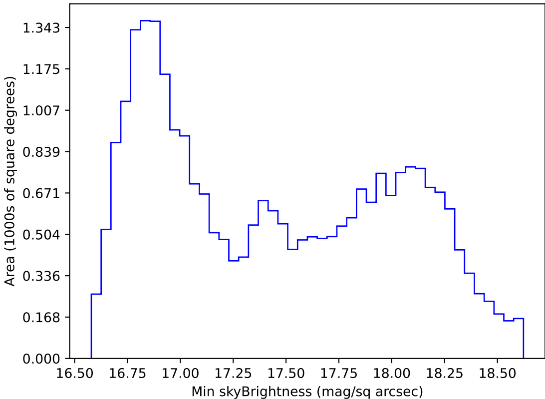
too_ignore_5_4v3.4_10yrs All sky z band: Min skyBrightness
