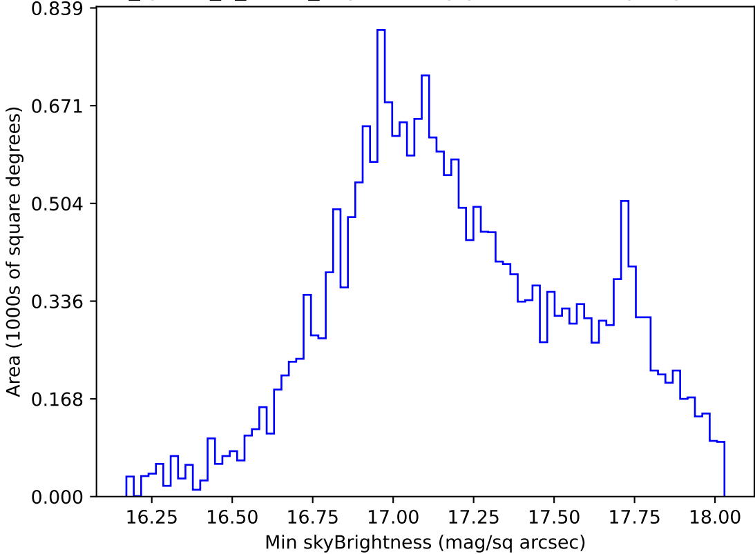
too_ignore_5_4v3.4_10yrs All sky y band: Min skyBrightness
