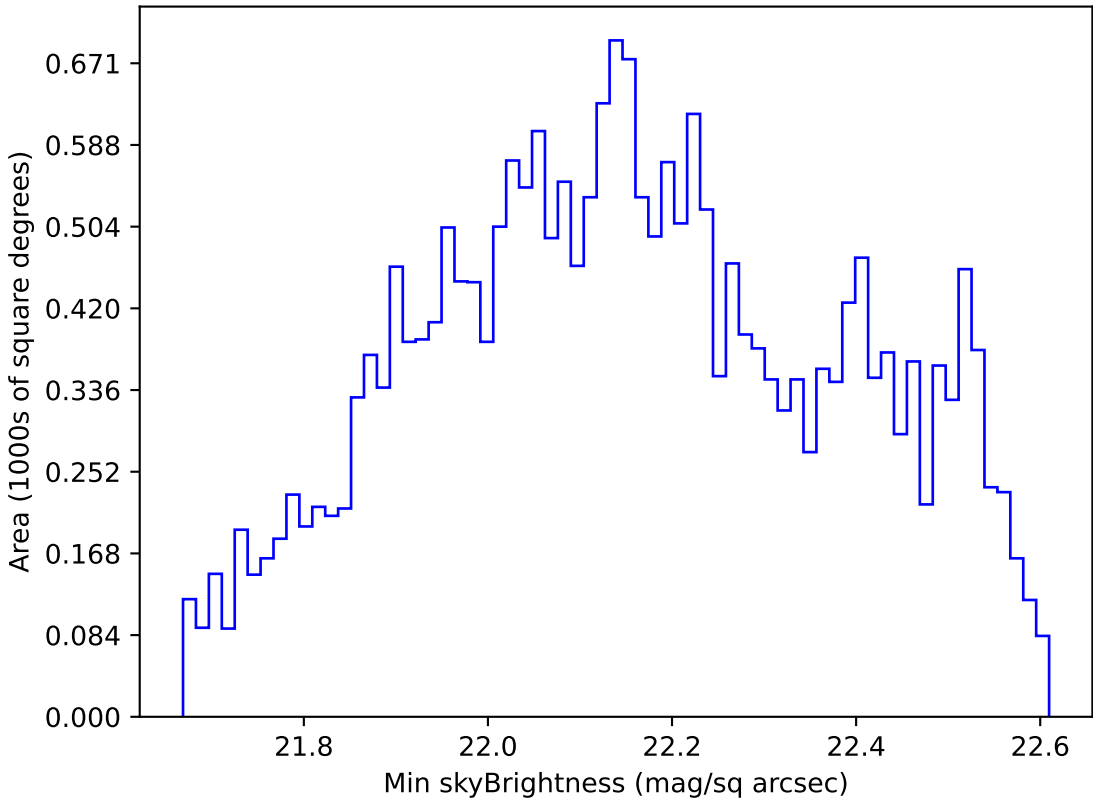
too_ignore_5_4v3.4_10yrs All sky u band: Min skyBrightness
