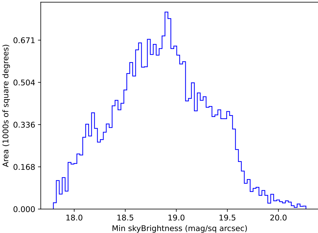
too_ignore_5_4v3.4_10yrs All sky r band: Min skyBrightness
