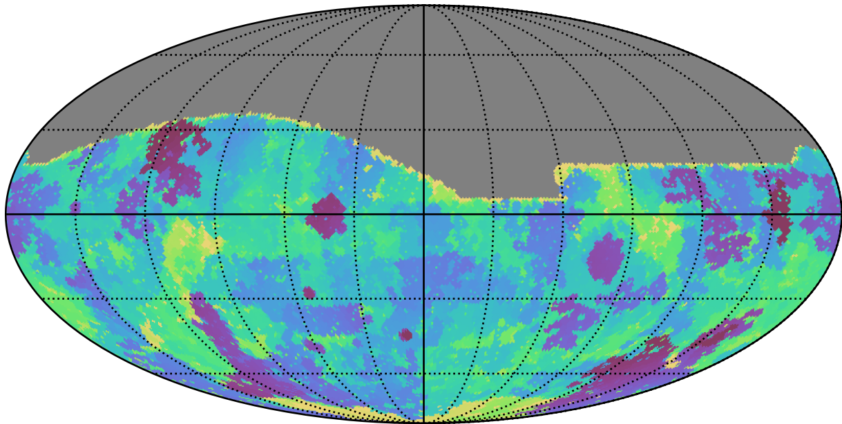
too_ignore_5_4v3.4_10yrs All sky g band: Min skyBrightness
