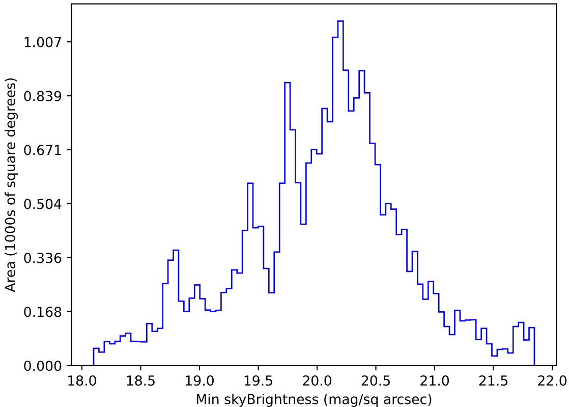
too_ignore_5_4v3.4_10yrs All sky g band: Min skyBrightness
