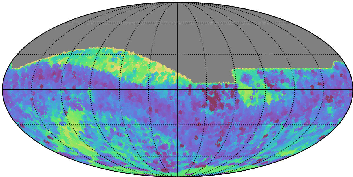
too_ignore_5_4v3.4_10yrs All sky all bands: Min skyBrightness
