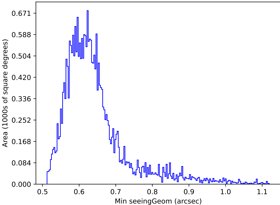
too_ignore_5_4v3.4_10yrs Yr 1 z band: Min seeingGeom
