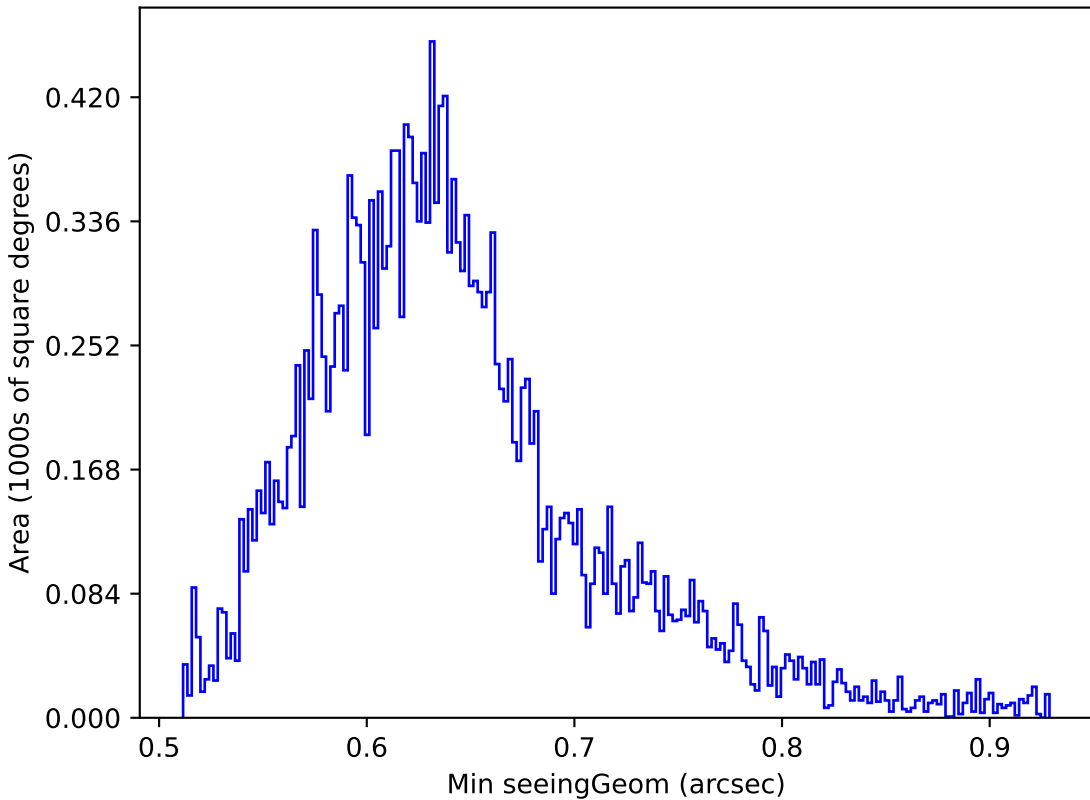
too_ignore_5_4v3.4_10yrs Yr 1 y band: Min seeingGeom
