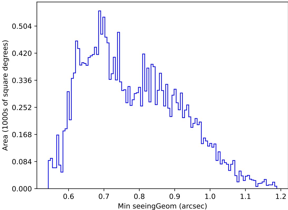
too_ignore_5_4v3.4_10yrs Yr 1 u band: Min seeingGeom
