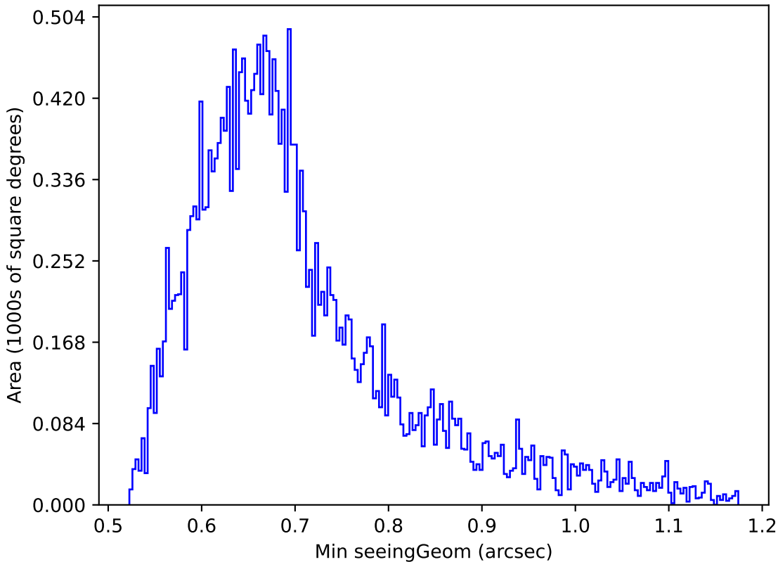
too_ignore_5_4v3.4_10yrs Yr 1 g band: Min seeingGeom
